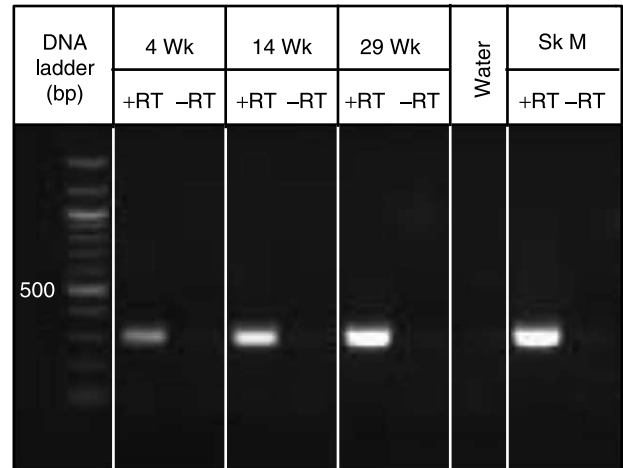
Figure 1 RT-PCR analysis of NAMPT gene expression in the testes of prepubertal and adult chickens. Total RNA was extracted, DNase-I digested, and RT (+RT). Approximately 50 ng of cDNA was used as template to amplify a 309-bp chicken NAMPT cDNA. Skeletal muscle cDNA was included as a positive control. Contamination controls consisted of RNA from each tissue without RT addition (-RT) or substitution of water for the cDNA template. 4 Wk, 4-week-old prepubertal chicken; 14 Wk, 14-week-old prepubertal chicken; 29 Wk, 29-week-old adult chicken, Sk M, skeletal muscle.
